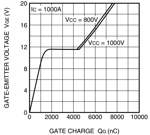
GATE CHARGE CHARACTERISTICS (TYPICAL)
